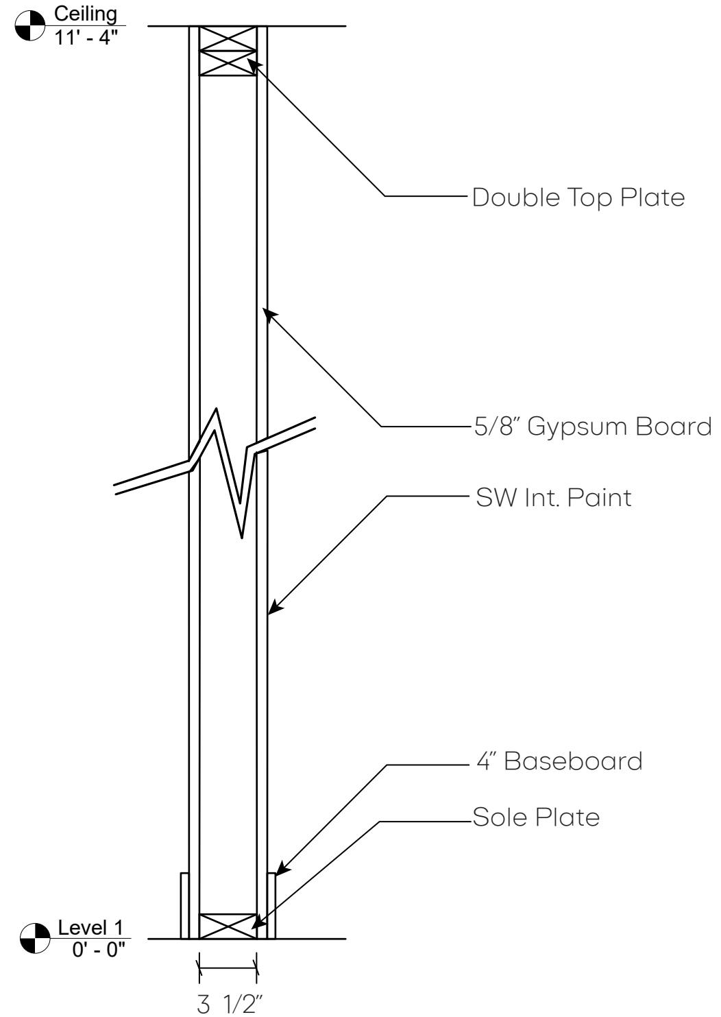
② Section 2 1 1/2" = 1'-0"
