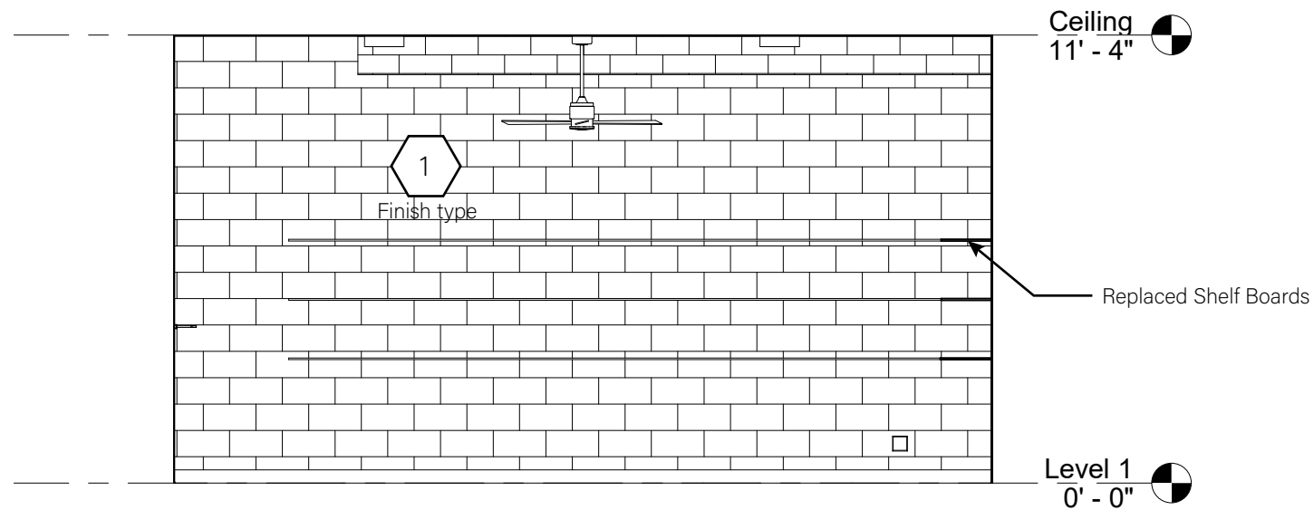
③ East Room-South Elevation 1/4" = 1'-0"
