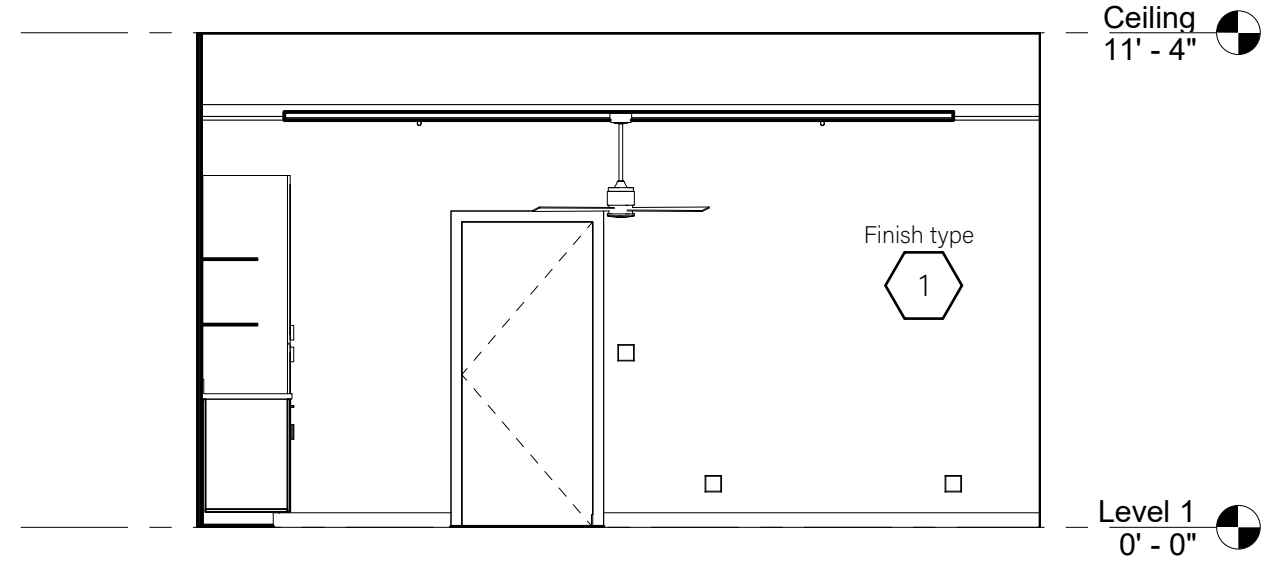
2 West Room-North Elevation 1/4" = 1'-0"
