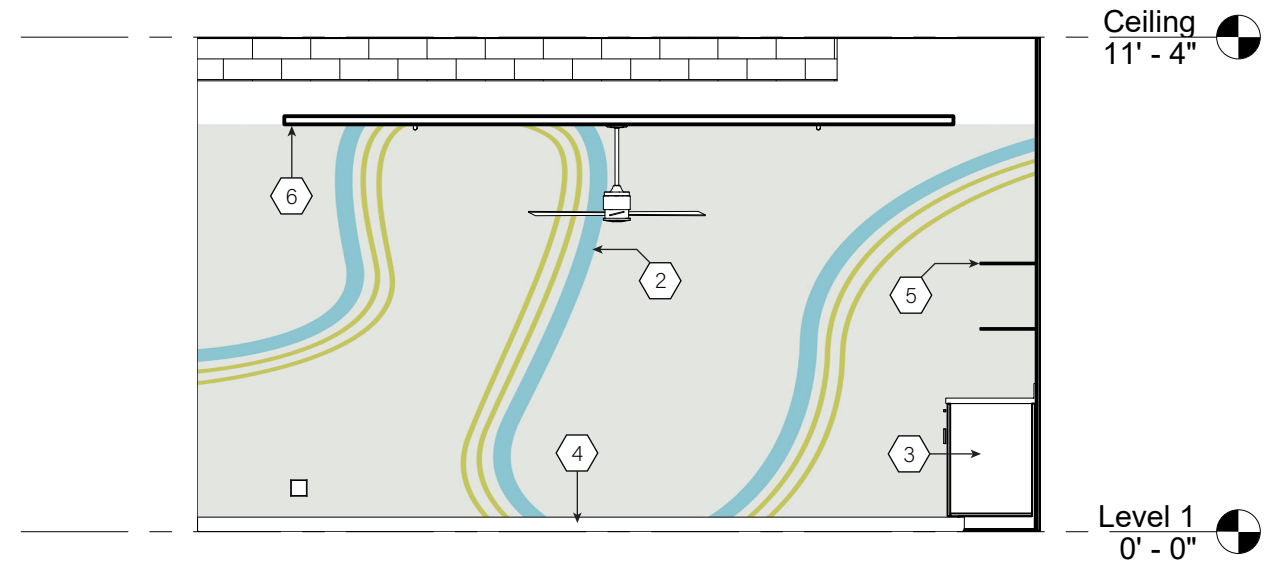
West Room - South Elevation
