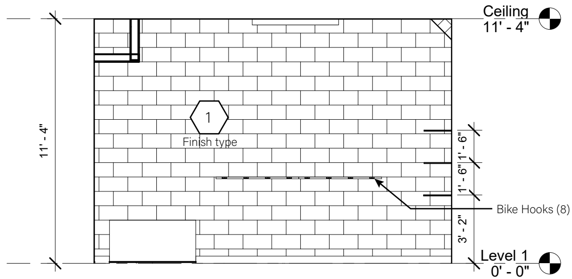
① East Room-East Elevation 1/4" = 1'-0"
