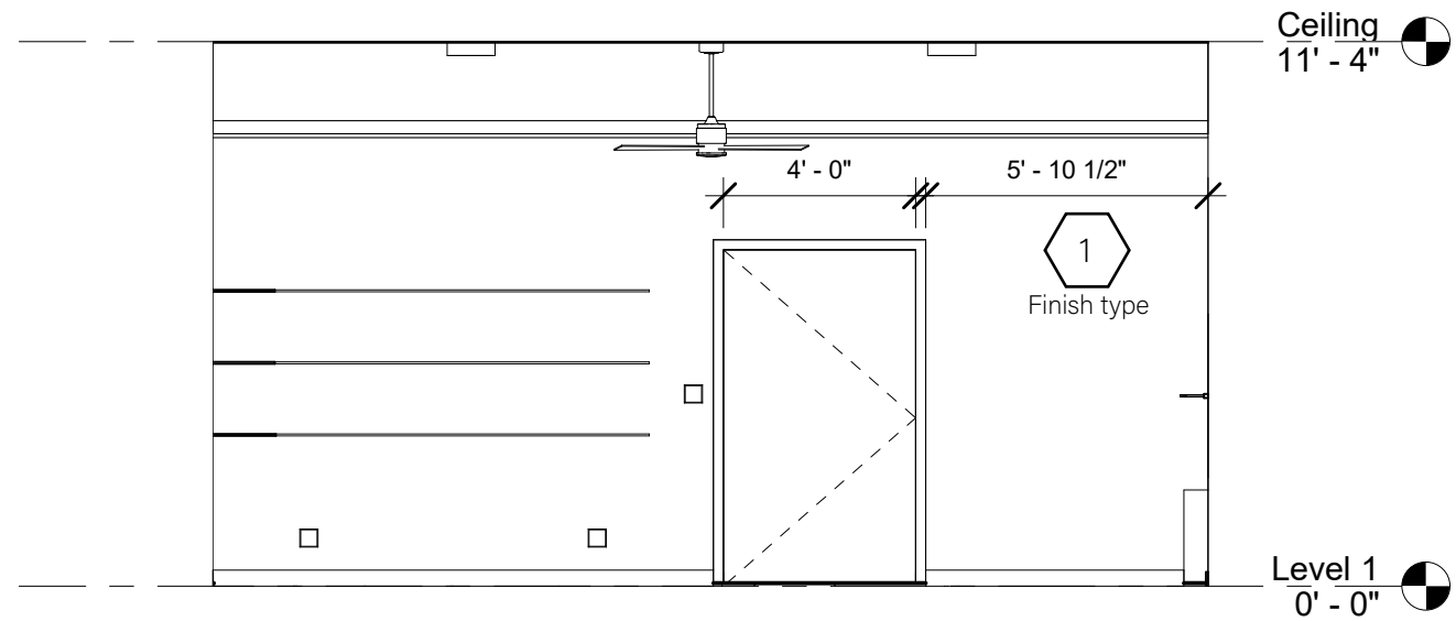
② East Room-North Elevation 1/4" = 1'-0"
