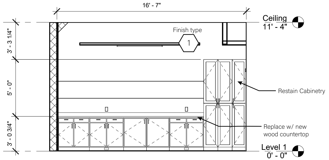
4 West Room-West View 1/4" = 1'-0"
