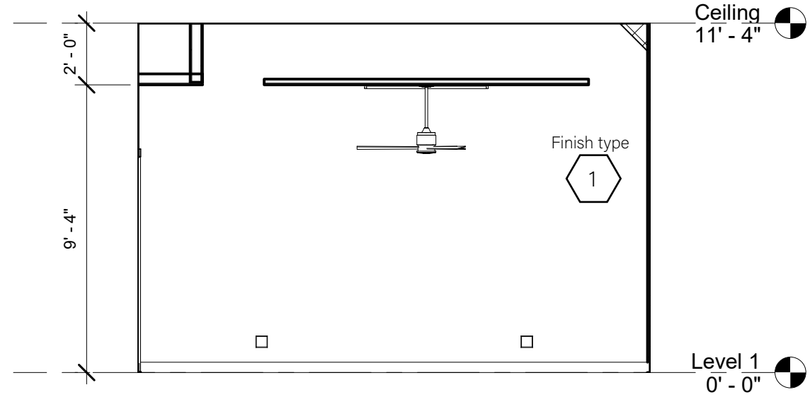
1 West Room-East Elevation 1/4" = 1'-0"
