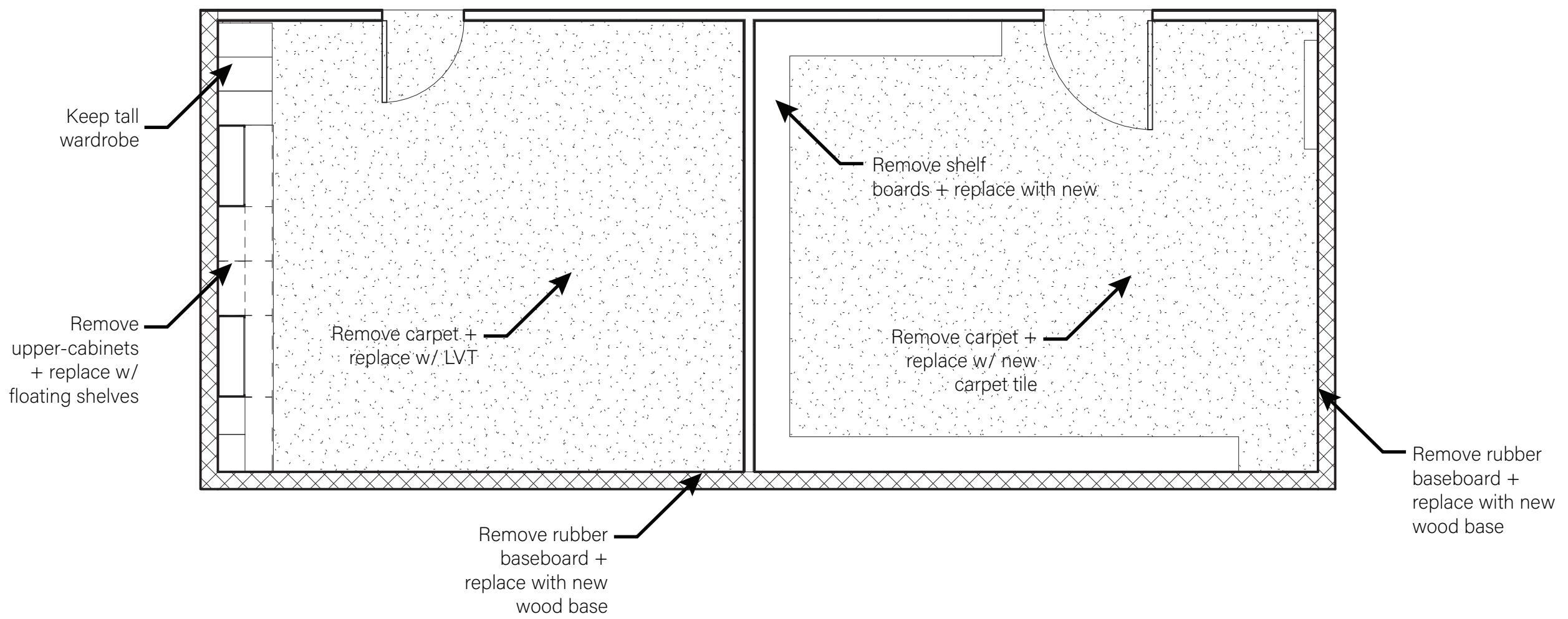
① Level 1 Demo Plan 1/4" = 1'-0"
