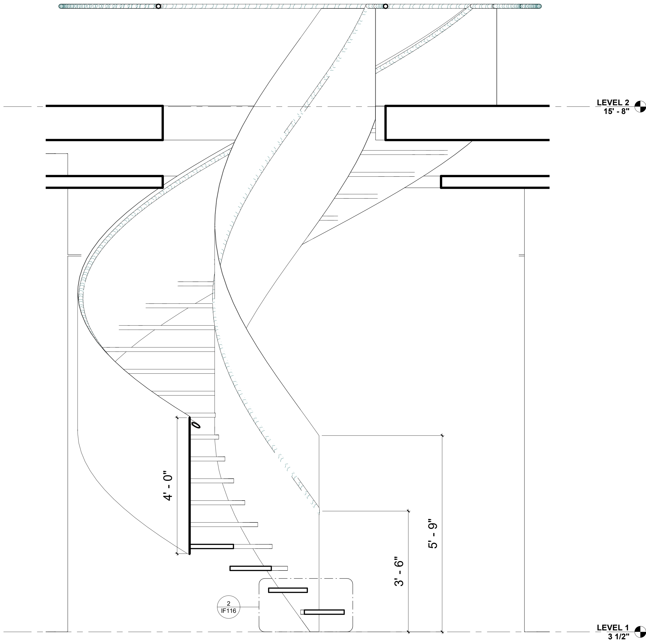
STAIRCASE SECTION
