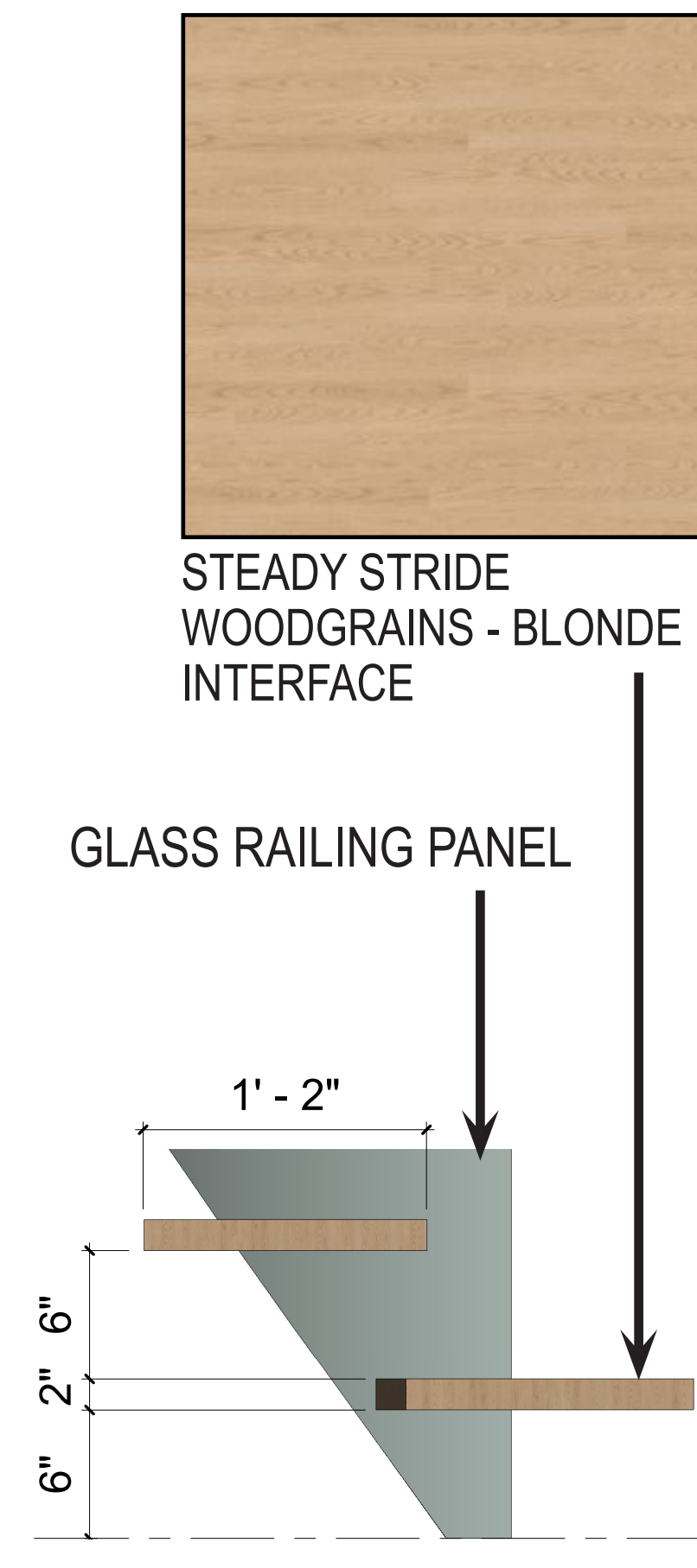
STAIR TREAD DETAIL
